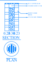
RAIN WATER HARVESTING 1.PERCOLATION PIT
