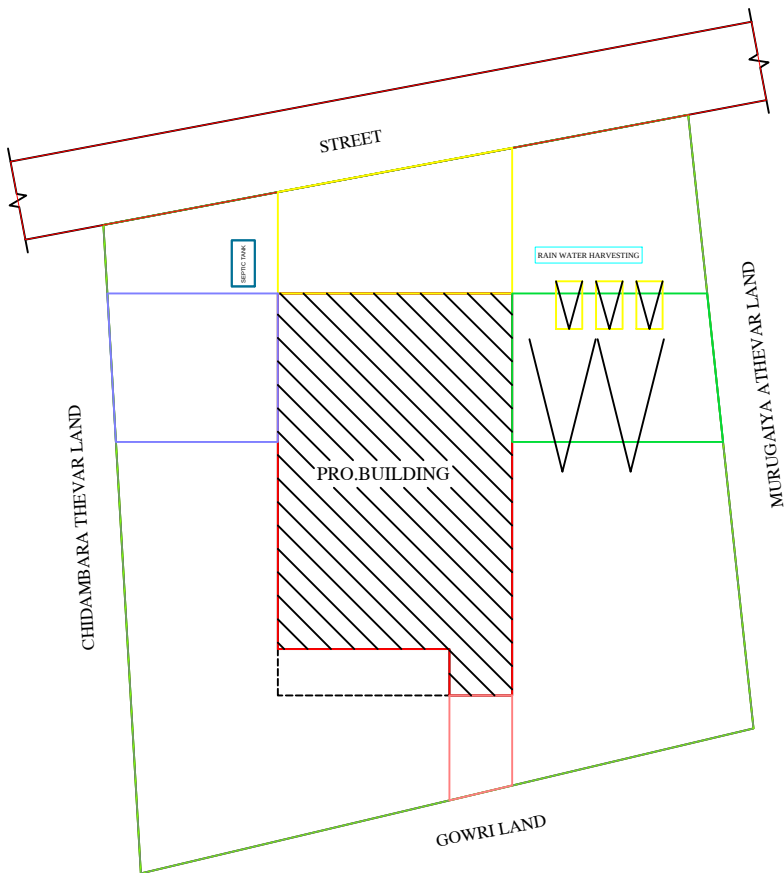
SITE PLAN
