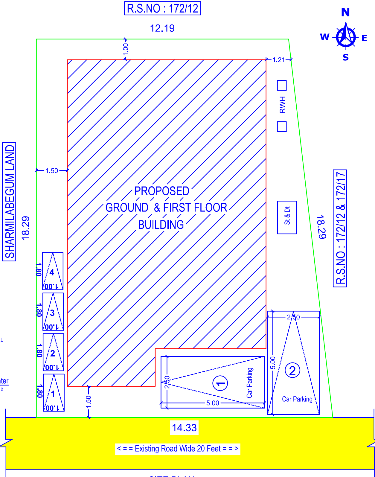
SITE PLAN
