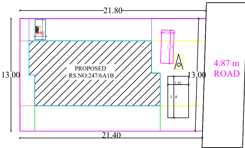
SITE PLAN
