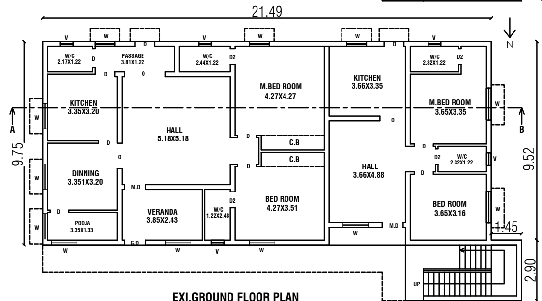
EXI.GROUND FLOOR PLAN
