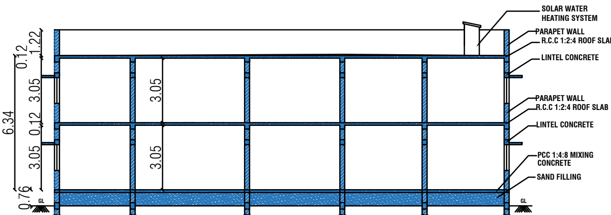
SECTION NO -"AB"
