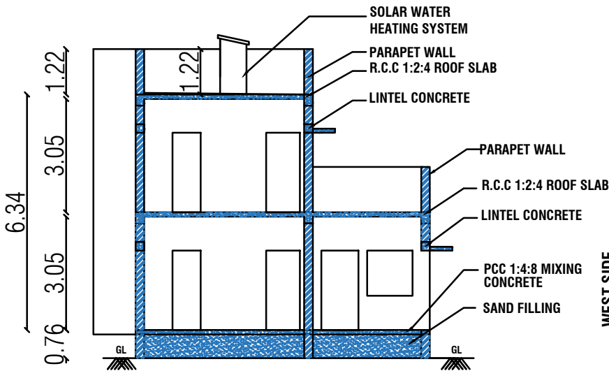
SECTION NO - "AB"
