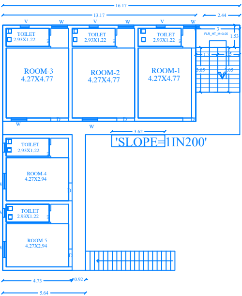
PRO-FIRST FLOOR PLAN BLOCK-3
