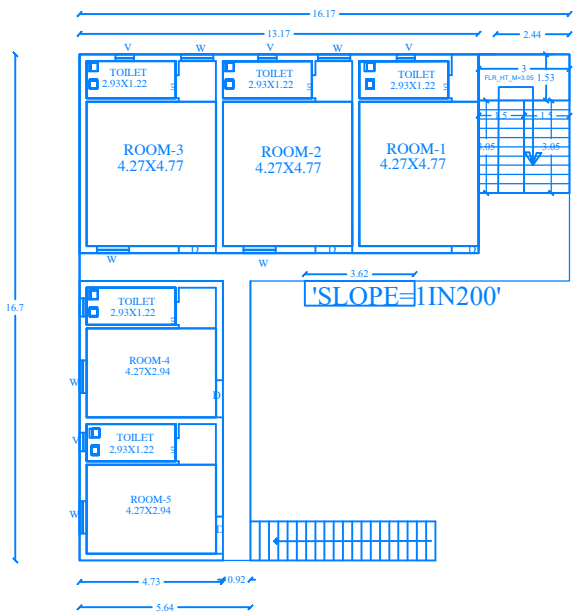
EXI-GROUND FLOOR PLAN BLOCK-3
