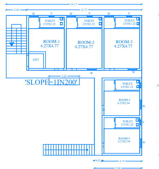
PRO-FIRST FLOOR PLAN BLOCK-4
