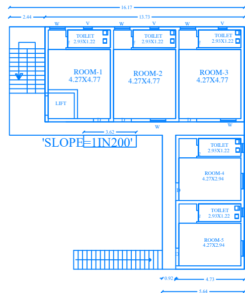
I-GROUND FLOOR PLAN BLOCK-4
