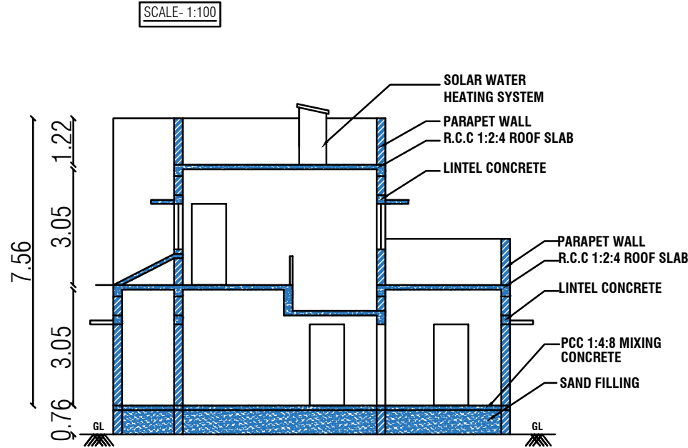
SECTION NO - "AB"
