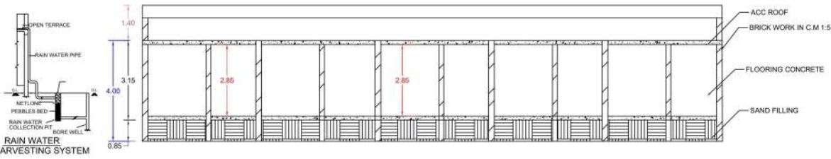
SECTION - XX-XX
