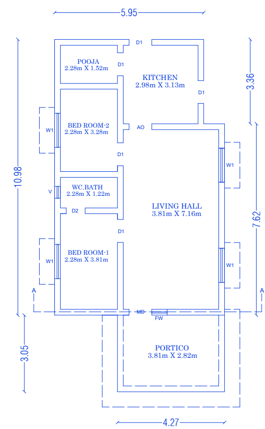
PRO-GROUND FLOOR
