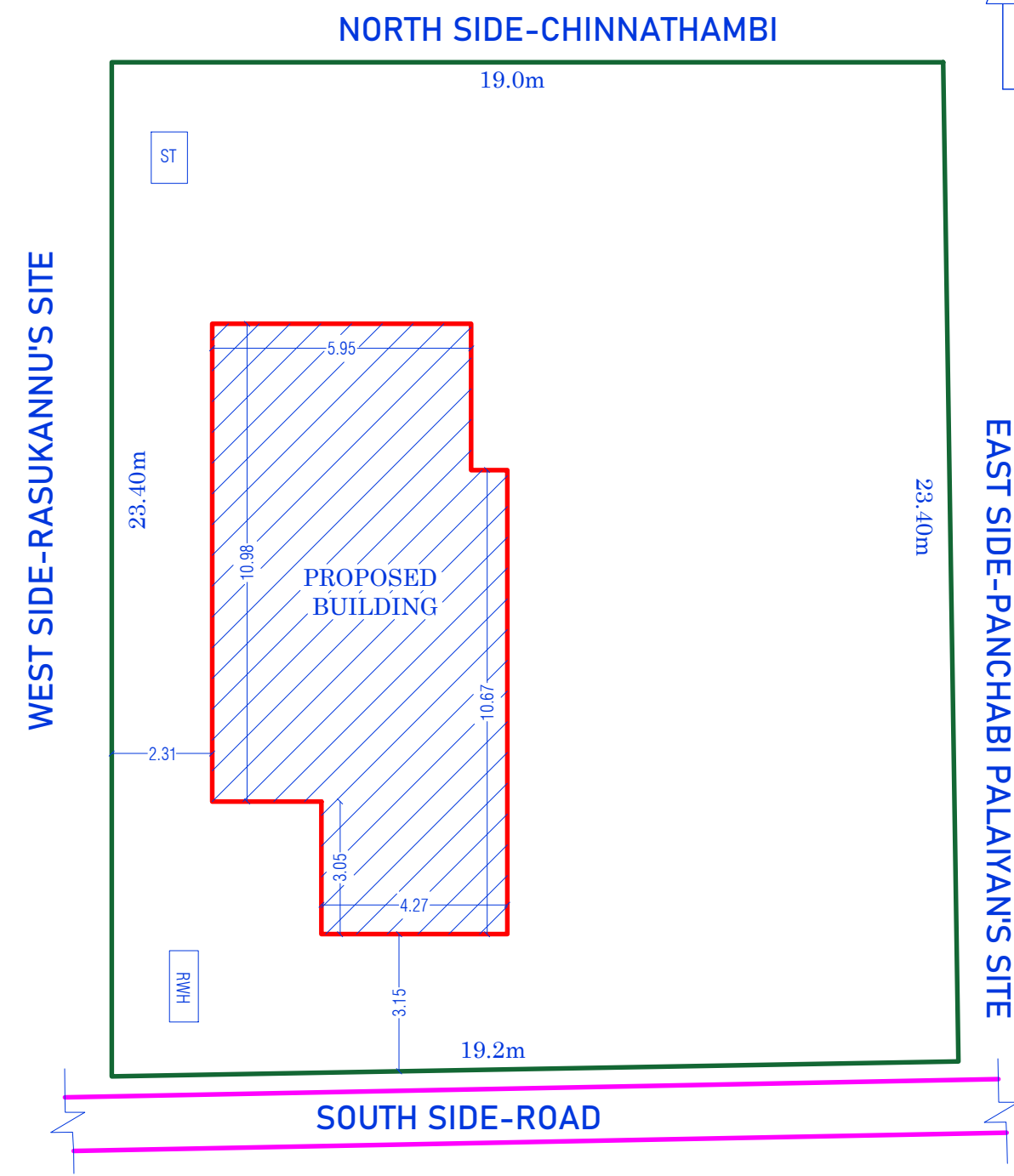
SITE PLAN
