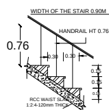
STAIR CASE STEPS SCALE 1:25
