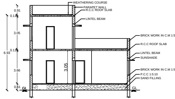
SECTION ON-XY
