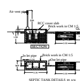
SEPTIC TANK DETAILS PLAN SCALE 1:50
