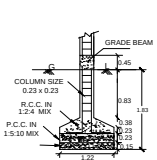
COLUMN DETAILS SCALE 1:25
