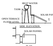
PLAN SOLAR WATER HEATER (NOT TO SCALE)
