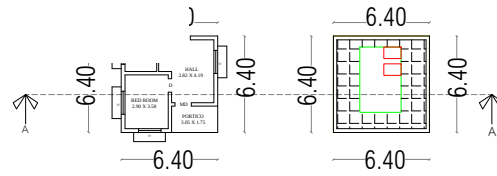
PRO.GROUND FLOOR PLAN
