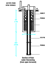
SECTION OF RAIN WATER HARVESTING (from open terrace)
