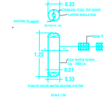
PLAN OF RAIN WATER HARVESTING SYSTEM SCALE 1:25
