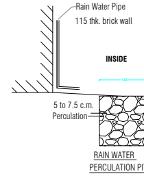
RAIN WATER PERCOLATION PIT
