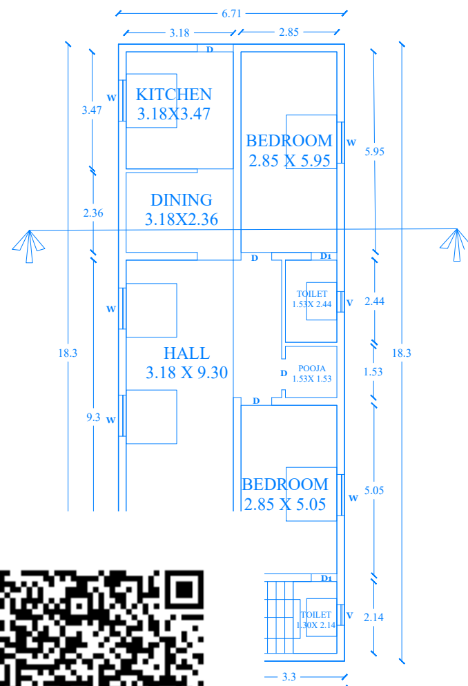
FLOOR PLAN
