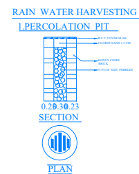
PLAN
