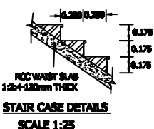
STAIR CASE DETAILS SCALE 1:25
