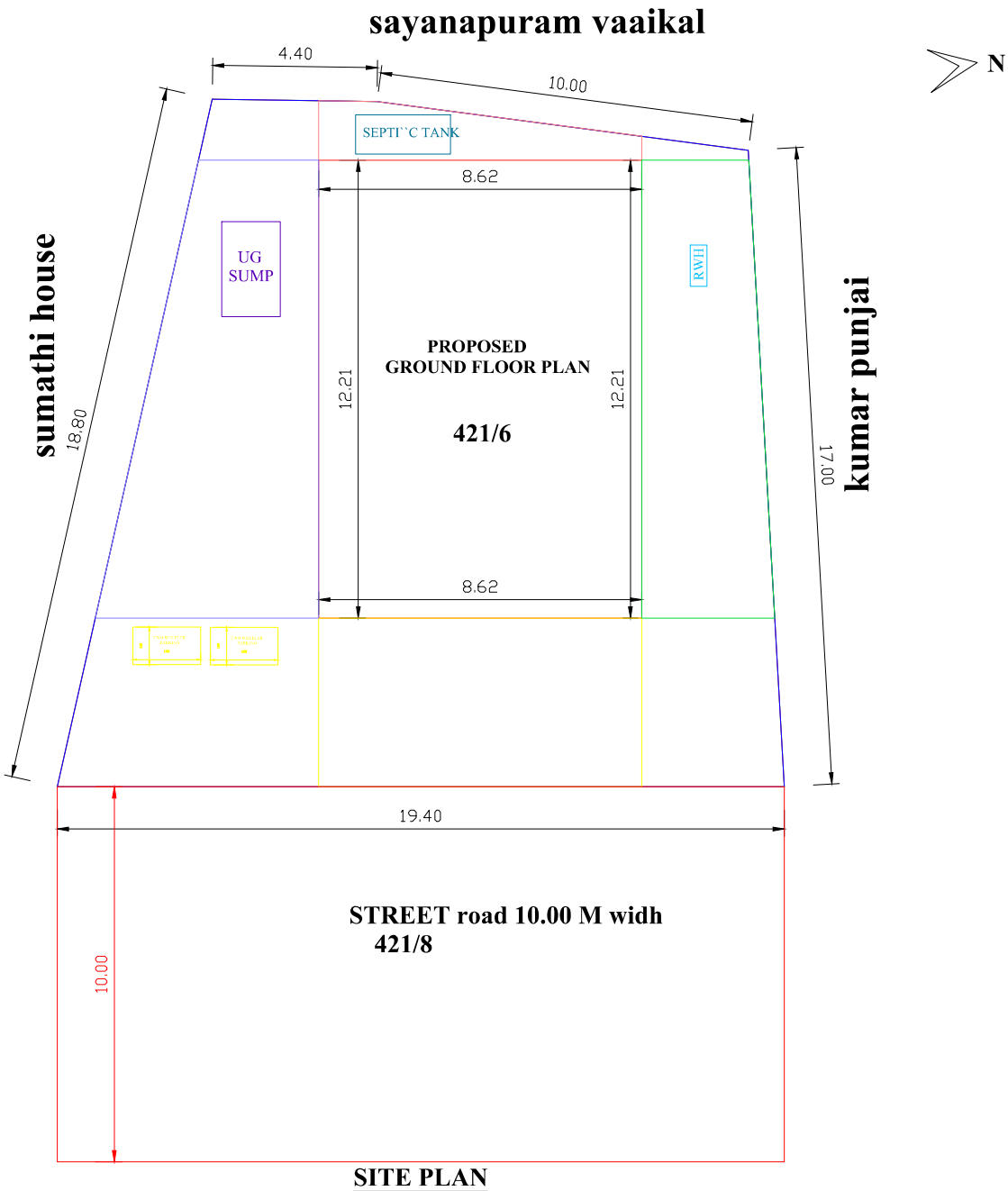
SITE PLAN
