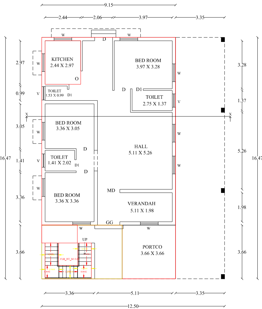
PRO & EXI. GROUND FLOOR
