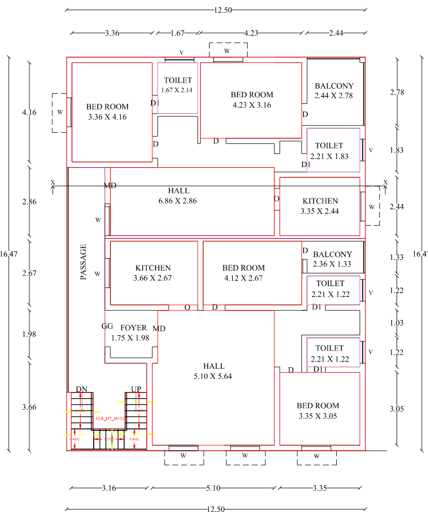
PRO FIRST FLOOR
