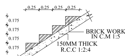
STAIRCASE DETAILS NOT TO SCALE
