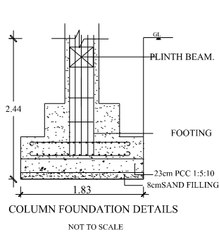
COLUMN FOUNDATION DETAILS NOT TO SCALE
