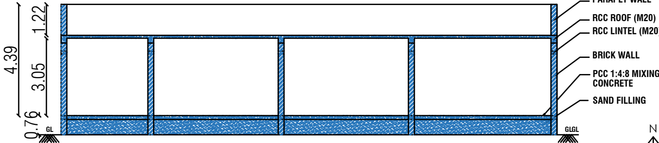
SECTION NO - "AB"
