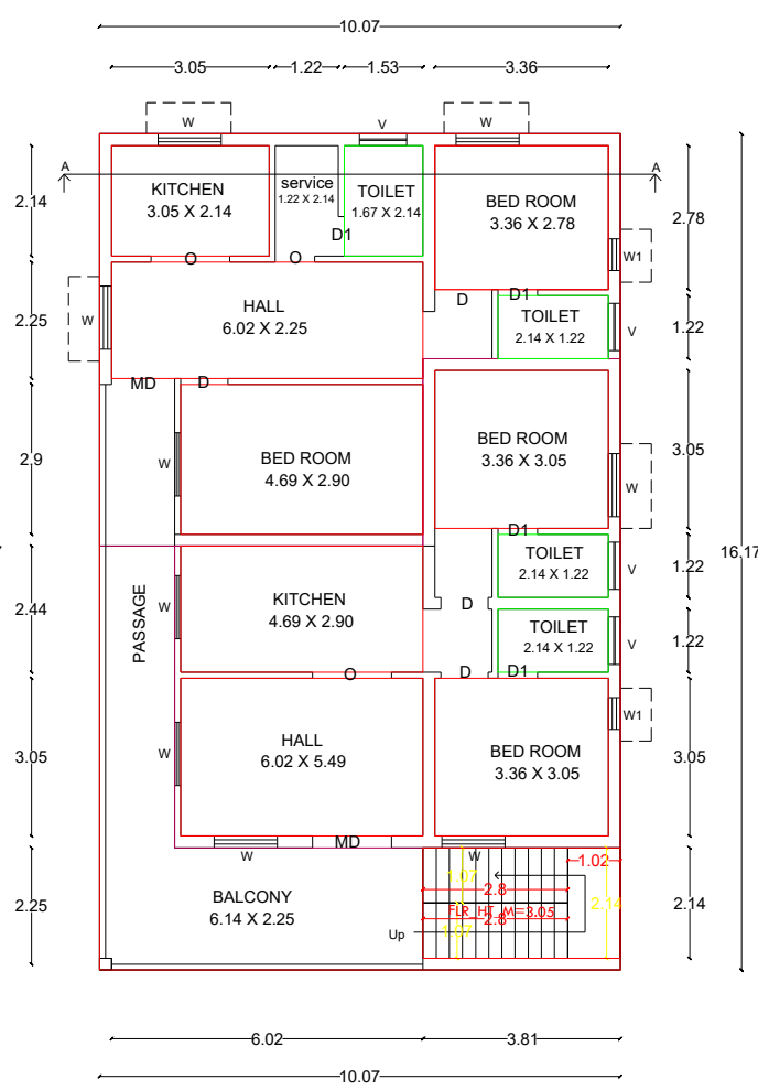
PRO FIRST FLOOR
