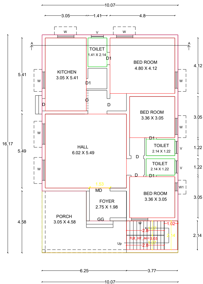
PRO.GROUND FLOOR
