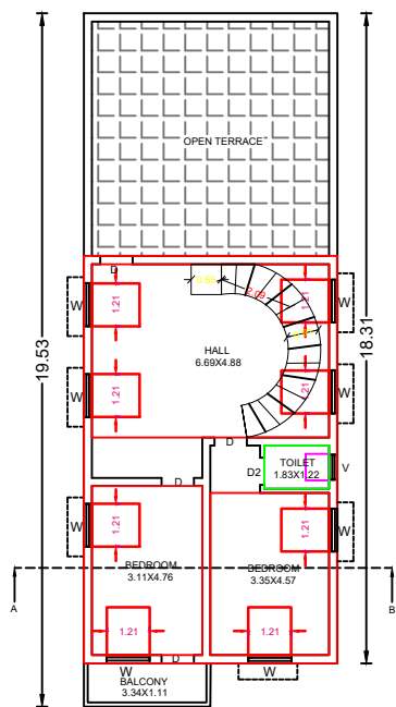
PRO.FIRST FLOOR PLAN
