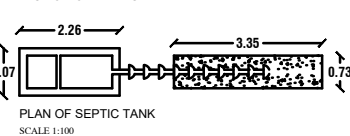
PLAN OF SEPTIC TANK SCALE 1:100
