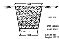
TRIAL PIT DETAILS NOT TO SCALE
