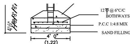
FOUNDATION DETAIL
