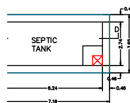
PLAN OF SEPTIC TANK SCALE 1"=2'0"
