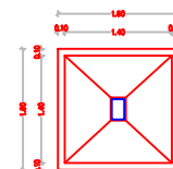
SECTION OF PEBBLE TRENCH
