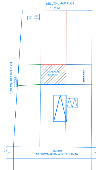
SITE PLAN SCALE 1:200
