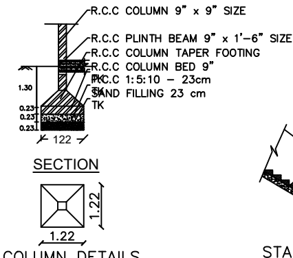
COLUMN DETAILS PLAN
