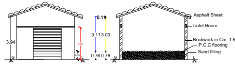
FRONT ELEVATION
