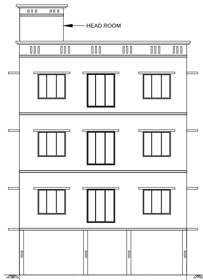
FRONT ELEVATION
