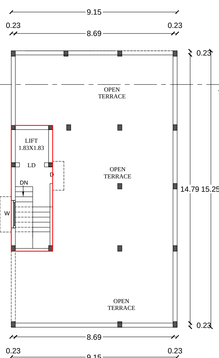
PRO- TERRACE FLOOR PLAN
