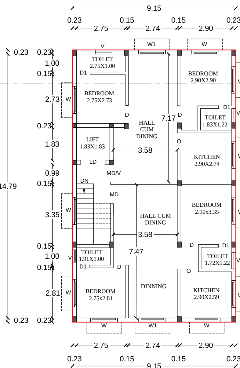
TYPICAL PRO- FIRST, SECOND & THIRD FLOOR PLAN
