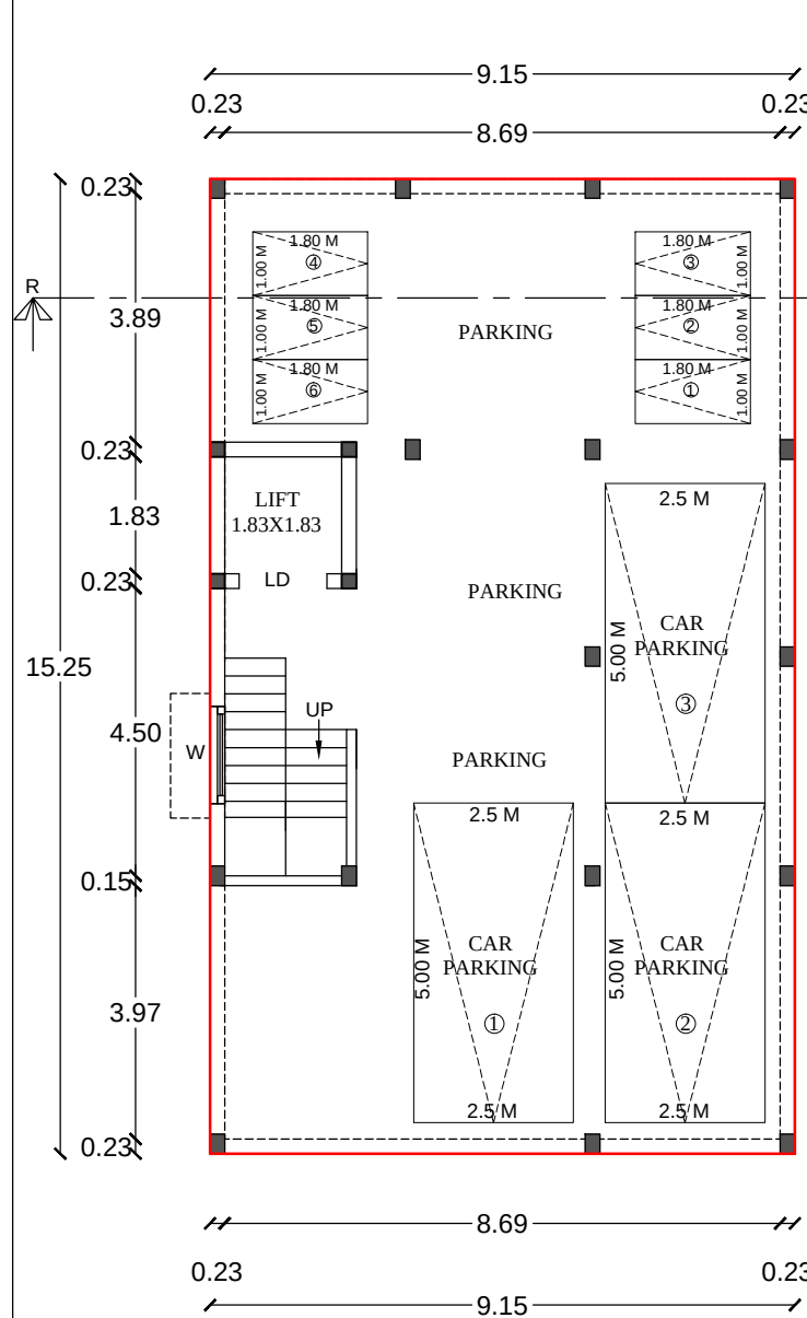
PRO- STILT FLOOR PLAN
