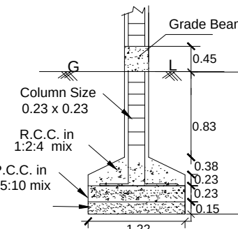
COLUMN DETAILS NOT TO SCALE
