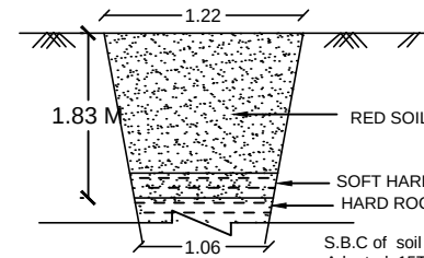
TRIAL PIT DETAILS NOT TO SCALE
