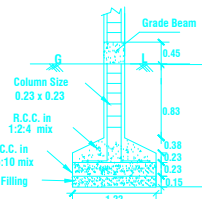
COLUMN DETAILS NOT TO SCALE
