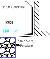
RAIN WATER PERCUSSION PIT
