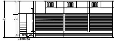
FRONT ELEVATION
