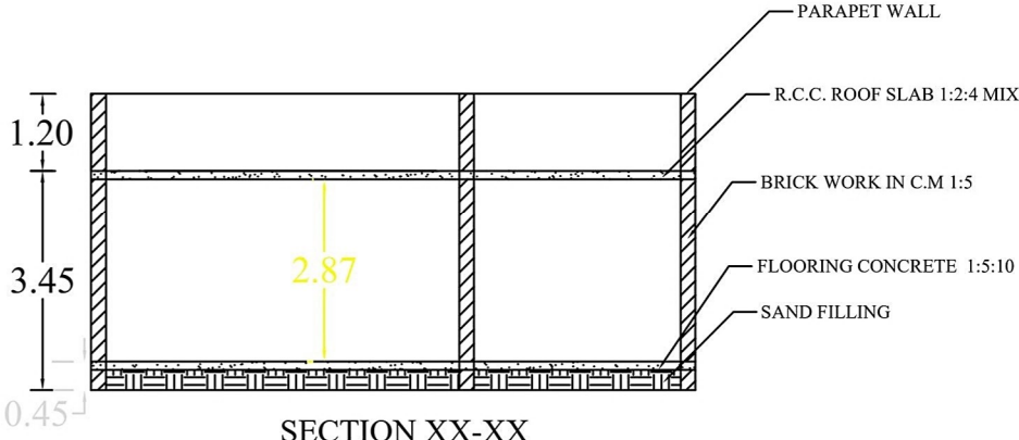
SECTION XX-XX
