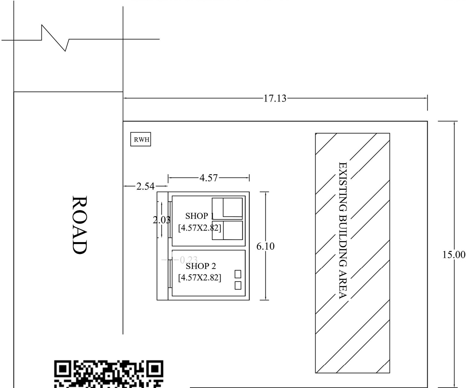
GROUND FLOOR
