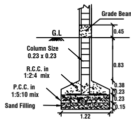
COLUMN DETAILS NOT TO SCALE
