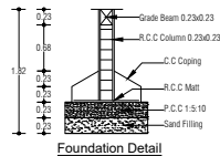
Foundation Detail
