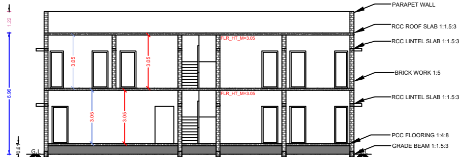
SECTION ON 'ABCD'
