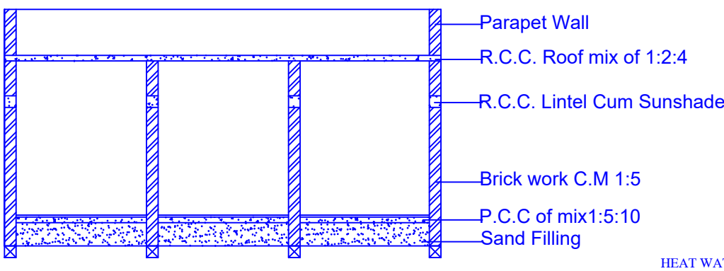
SECTION ON RS
