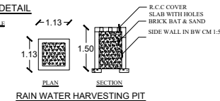
RAIN WATER HARVESTING PIT
