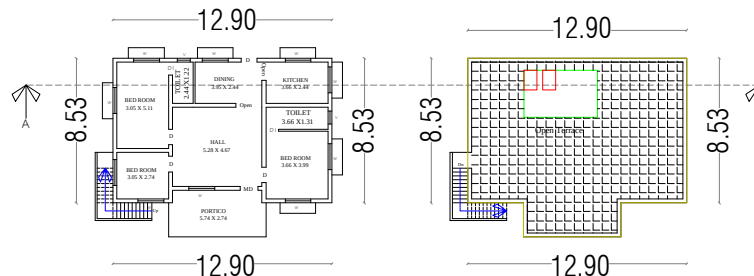
PRO.GROUND FLOOR PLAN
