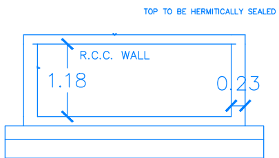
RWH_SECTION (SAMPLE)
