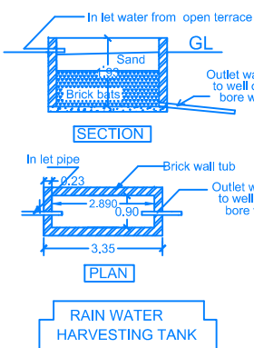
RAIN WATER HARVESTING TANK
