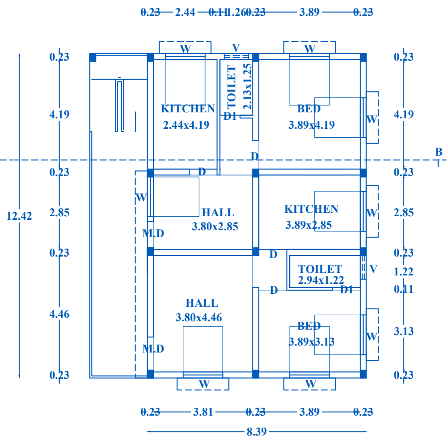
FLOOR-01
