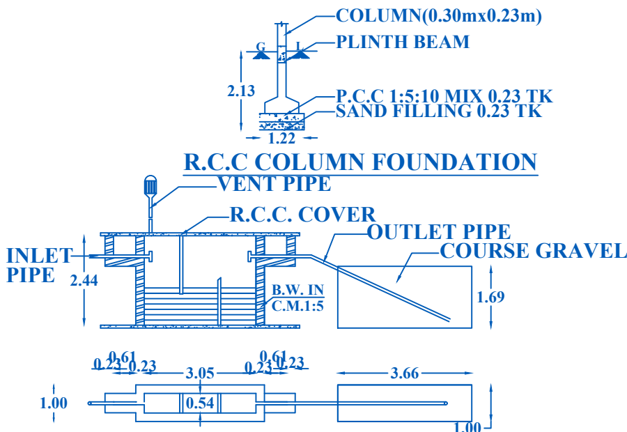
SEPTIC TANK & OF DISPERSION TRENCH DETAILS (NOT TO SCALE)
