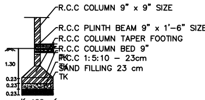
SECTION
