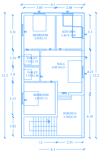
ND FLOOR PLAN
