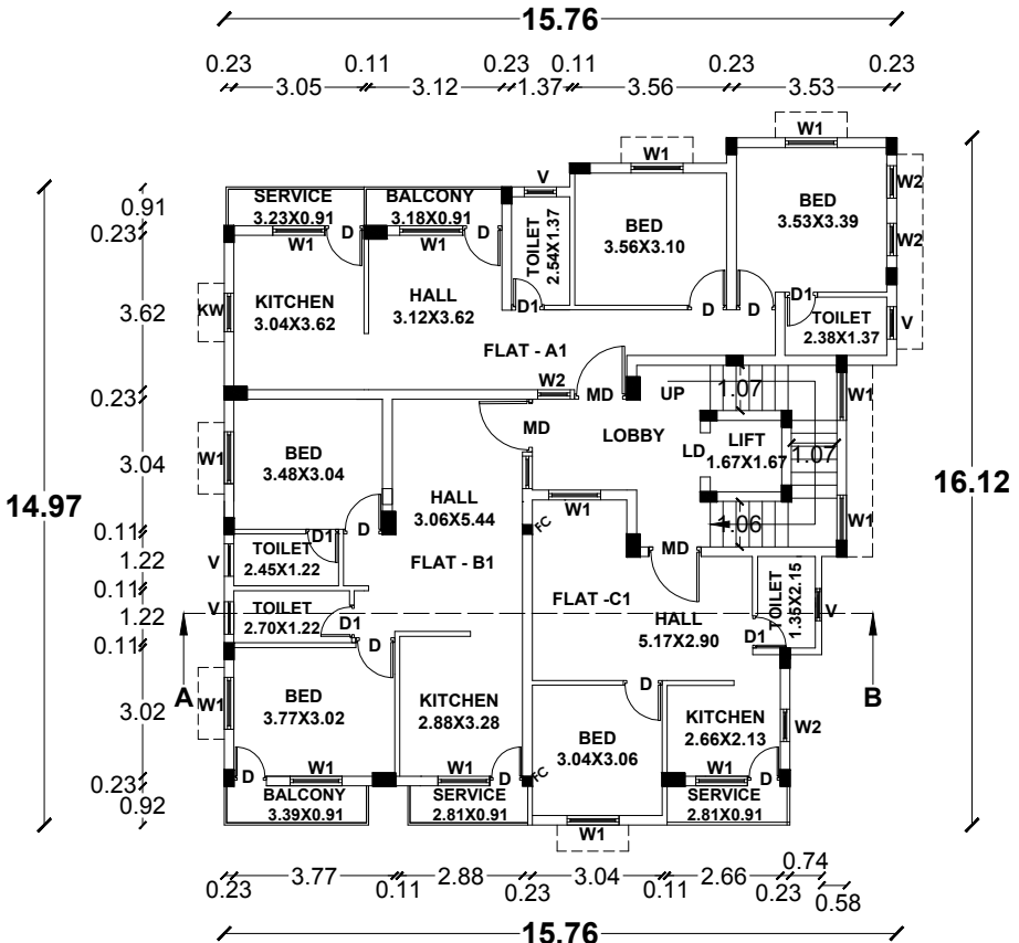
FIRST FLOOR & SECOND FLOOR-TYPICAL FLOOR PLAN
