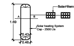
PLAN OF SOLAR WATER HEATING SYSTEM
