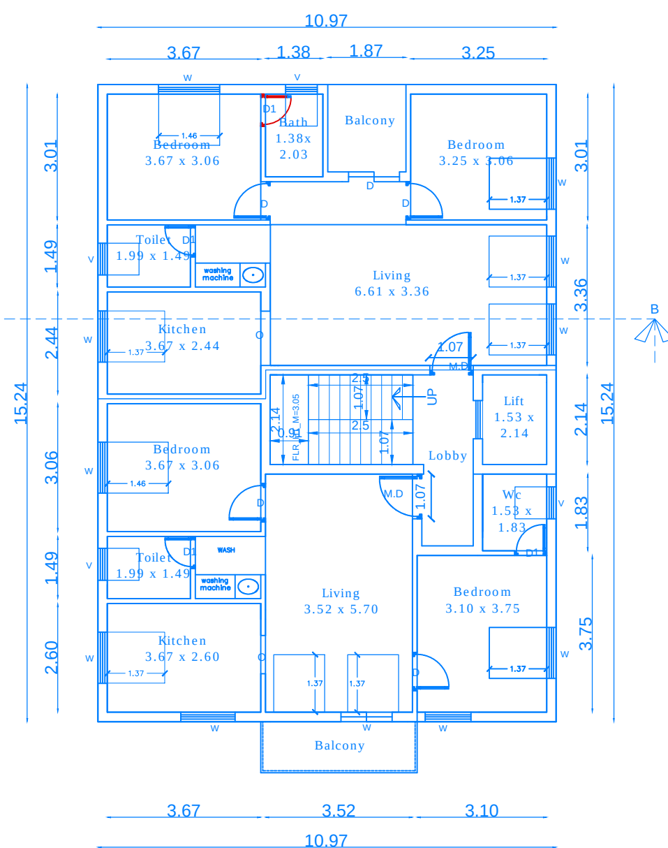
TYPICAL FIRST, SECOND & THIRD FLOOR PLAN
