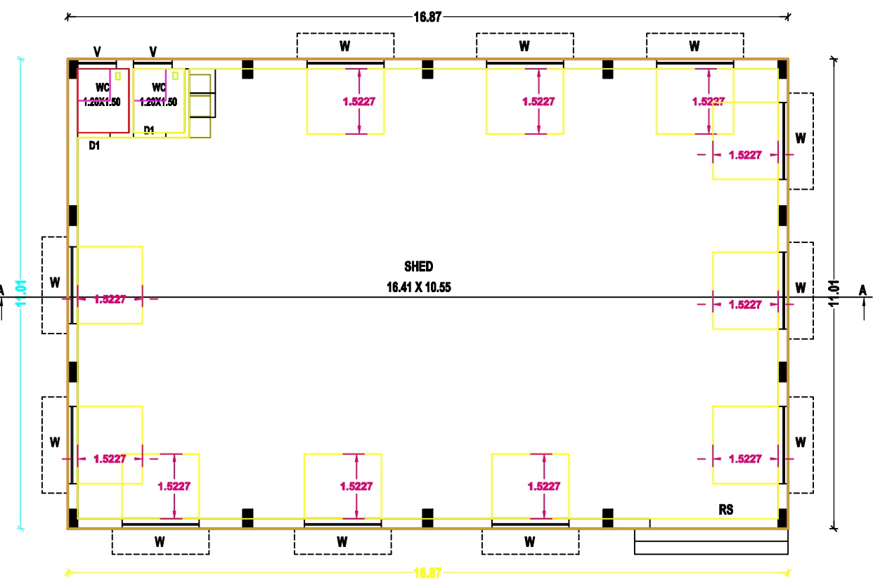
Floor plan
