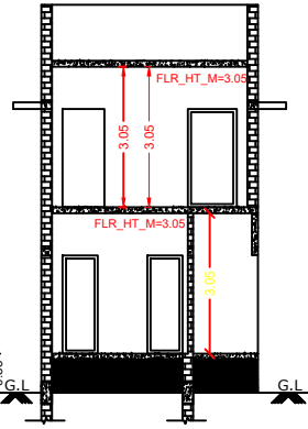
SECTION ON 'ABCD'
