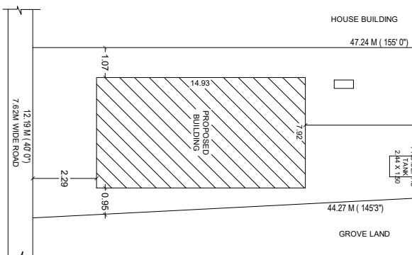
SITE PLAN
