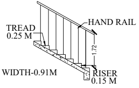
STAIRCASE DETAILS
