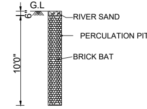
PERCOLATION PIT
