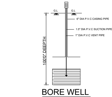
BORE WELL
