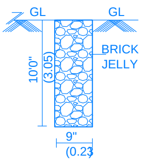
PERCOLATION PIT
