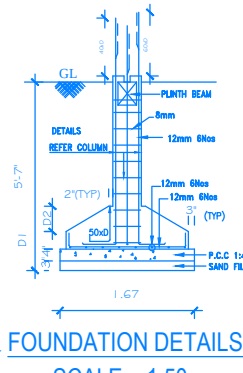
FOUNDATION DETAILS SCALE : 1:50
