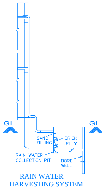
RAIN WATER HARVESTING SYSTEM
