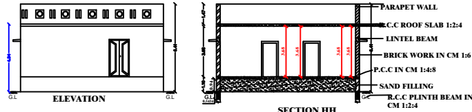
SECTION HH
