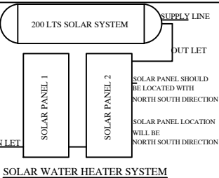
SOLAR WATER HEATER SYSTEM
