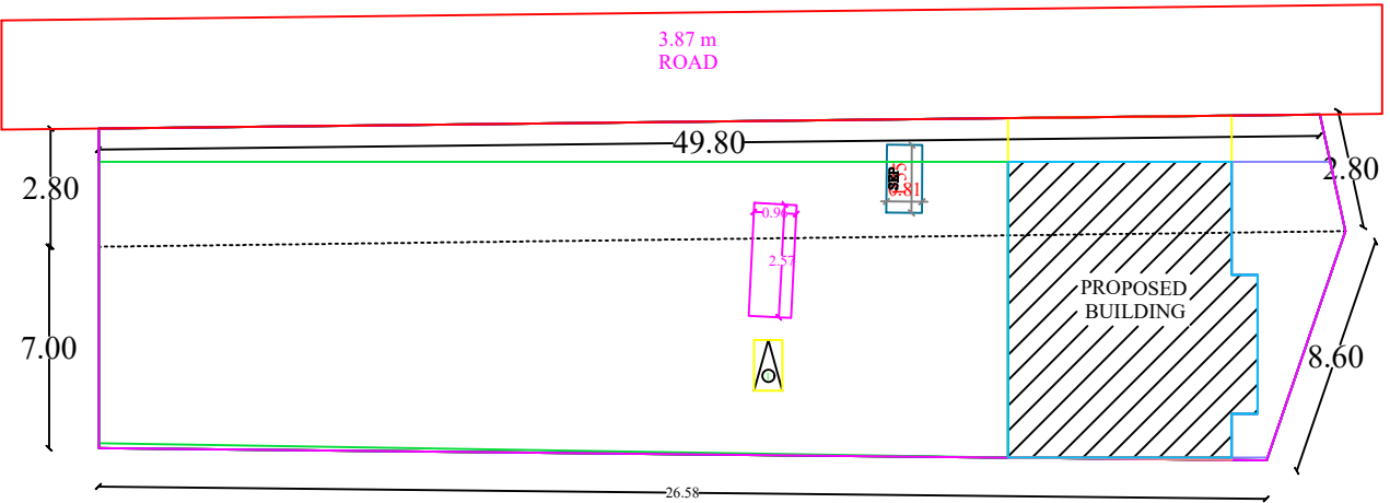
SITE PLAN
