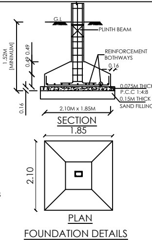
FOUNDATION DETAILS
